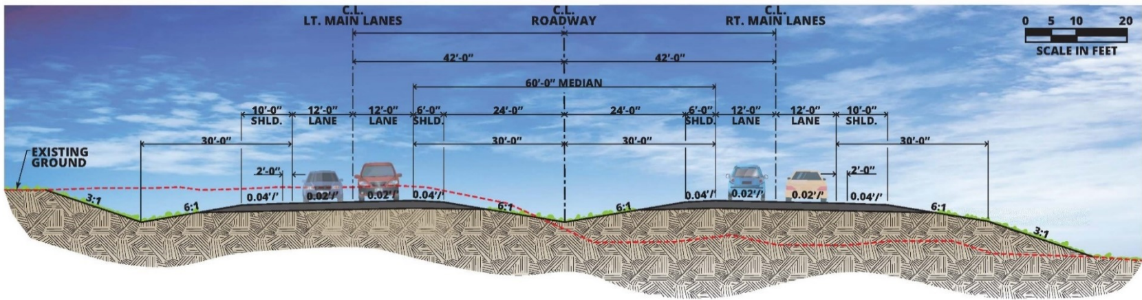
XNA ACCESS TYPICAL DIVIDED HIGHWAY SECTION NEW LOCATION ALTERNATIVE
