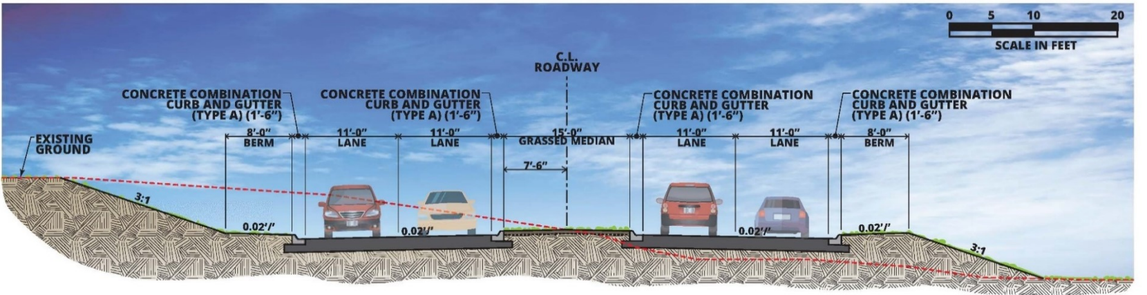
XNA ACCESS TYPICAL CURB & GUTTER SECTION PARTIAL NEW LOCATION ALTERNATIVE IMPROVE EXISTING ALTERNATIVE
